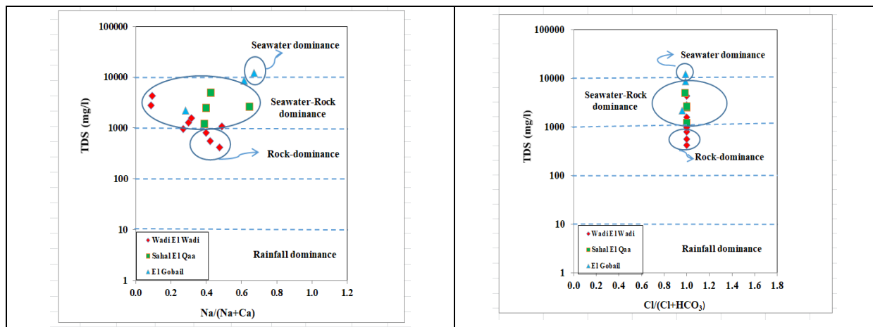
Fig (6): Gibbs plot for collected groundwater samples.
