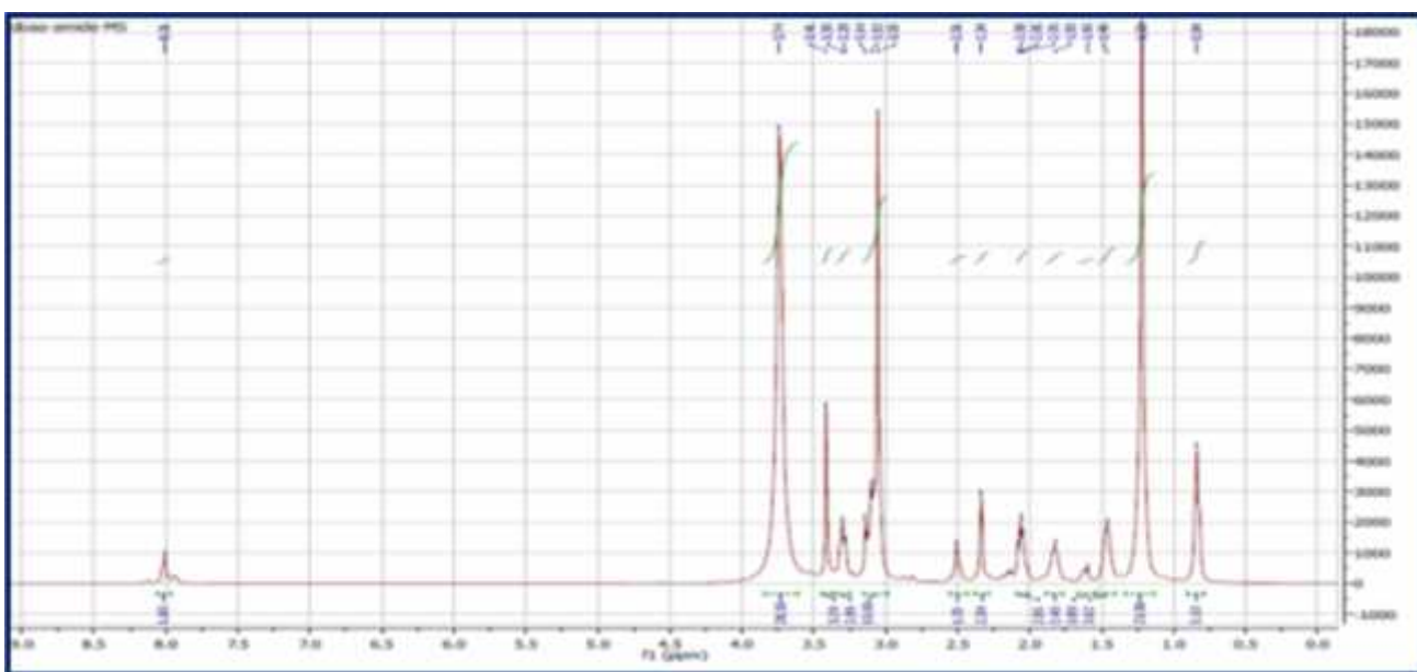
Fig (4): 1 H NMR spectra of 3-Decanoylamino-Propyl-Ethyl-Dimethyl-Ammonium Iodide (DAEI).
