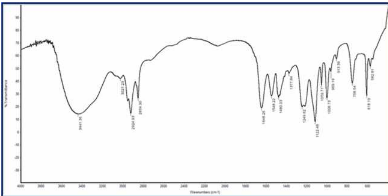
Fig (3): FT-IR spectra of 3-Decanoylamino-Propyl-Ethyl-Dimethyl-Ammonium Iodide (DAEI).
