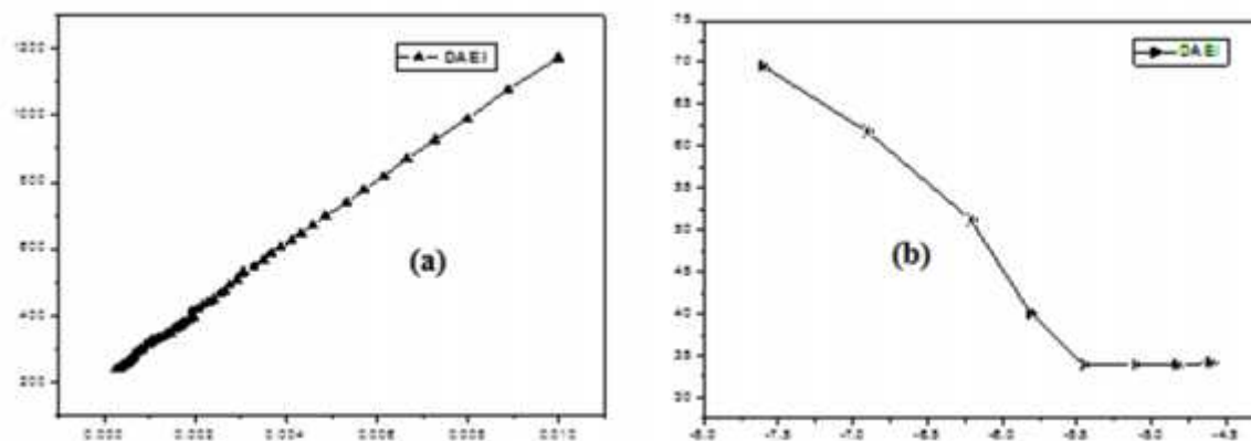
Fig (5): (a) The relation between electrical conductivity and concentration of DAEI at 298 K. (b) The relation between surface tension and -\log concentration of DAEI at 298 K.
