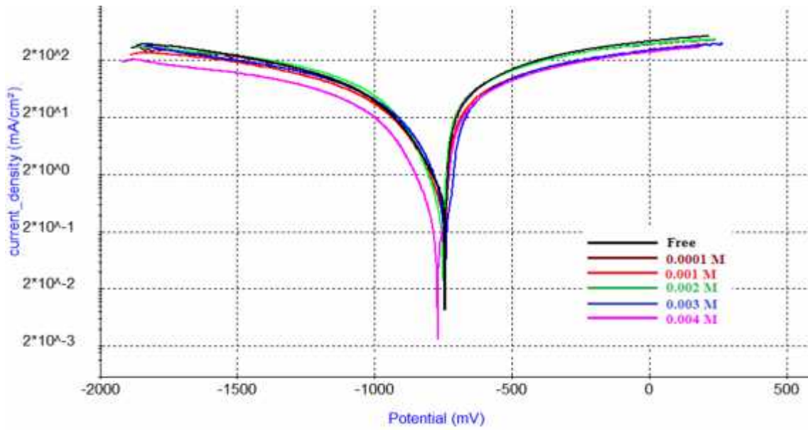
Fig (8): Anodic and cathodic polarization curves for aluminum 1050 in 0.5 M HCl solution and different concentrations of the surfactant (DAEI), at room temperature and scan rate of 1 mV/sec.
